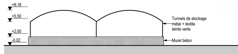
FACADE SUD
